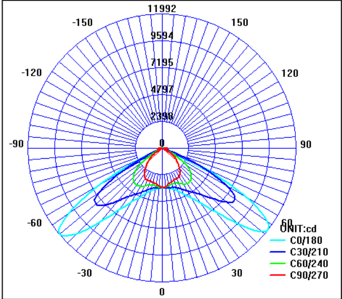
Batwing Light Distribution
