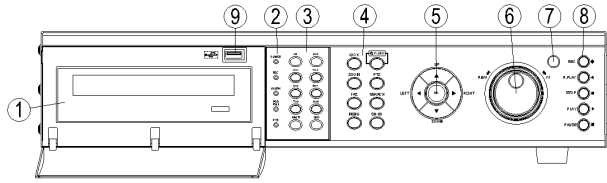
Figure 1. 16CH DVR Front
