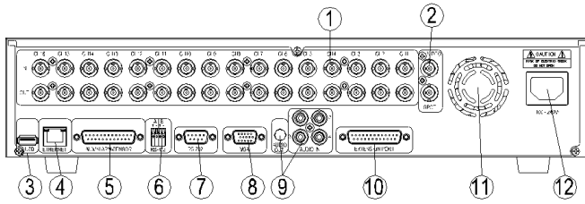
Figure 4. 16CH DVR Rear panel
