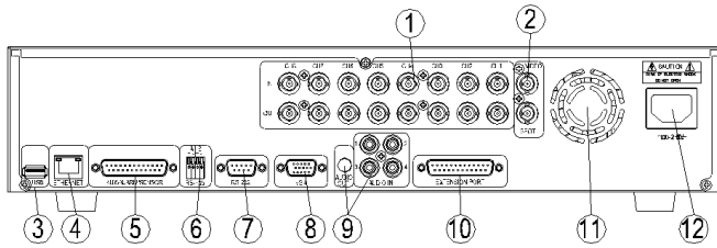
Figure 5. 8CH DVR Rear panel
