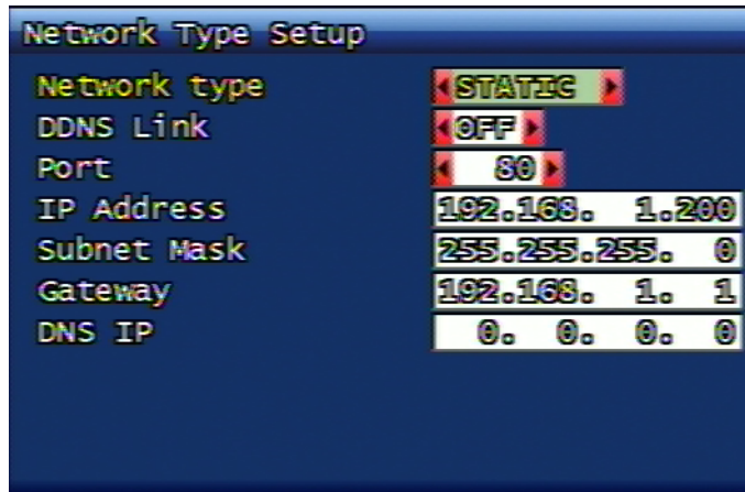
Figure 3.31. Static Setup Screen
